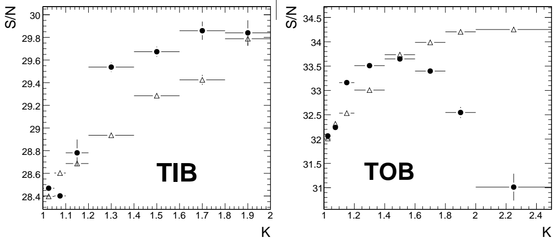
Figure 20: S_{ren}/N dependence on K for tracks perpendicular to the strip direction (open triangles) , i.e. the XZ local direction, and for tracks parallel to the strip direction (black circles) , i.e. the YZ local direction, for TIB and TOB.
