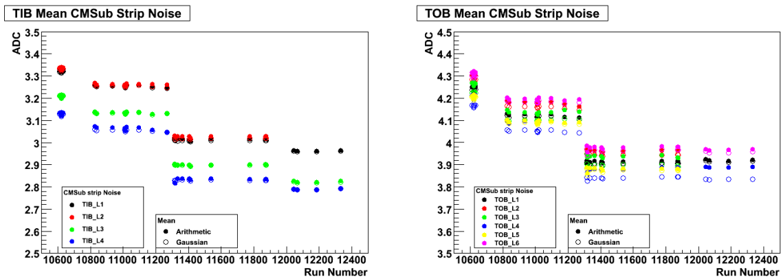
Figure 11: Noise vs run number for TIB on the left and for TOB on the right. Four periods at different temperatures are visible: 10^{\circ}\text{C} , 0^{\circ}\text{C} , -10^{\circ}\text{C} and -15^{\circ}\text{C}
